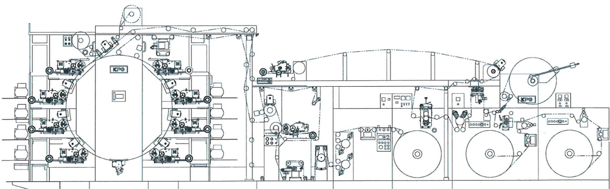
10-colour UV flexo printing including flexo varnish and foiling
